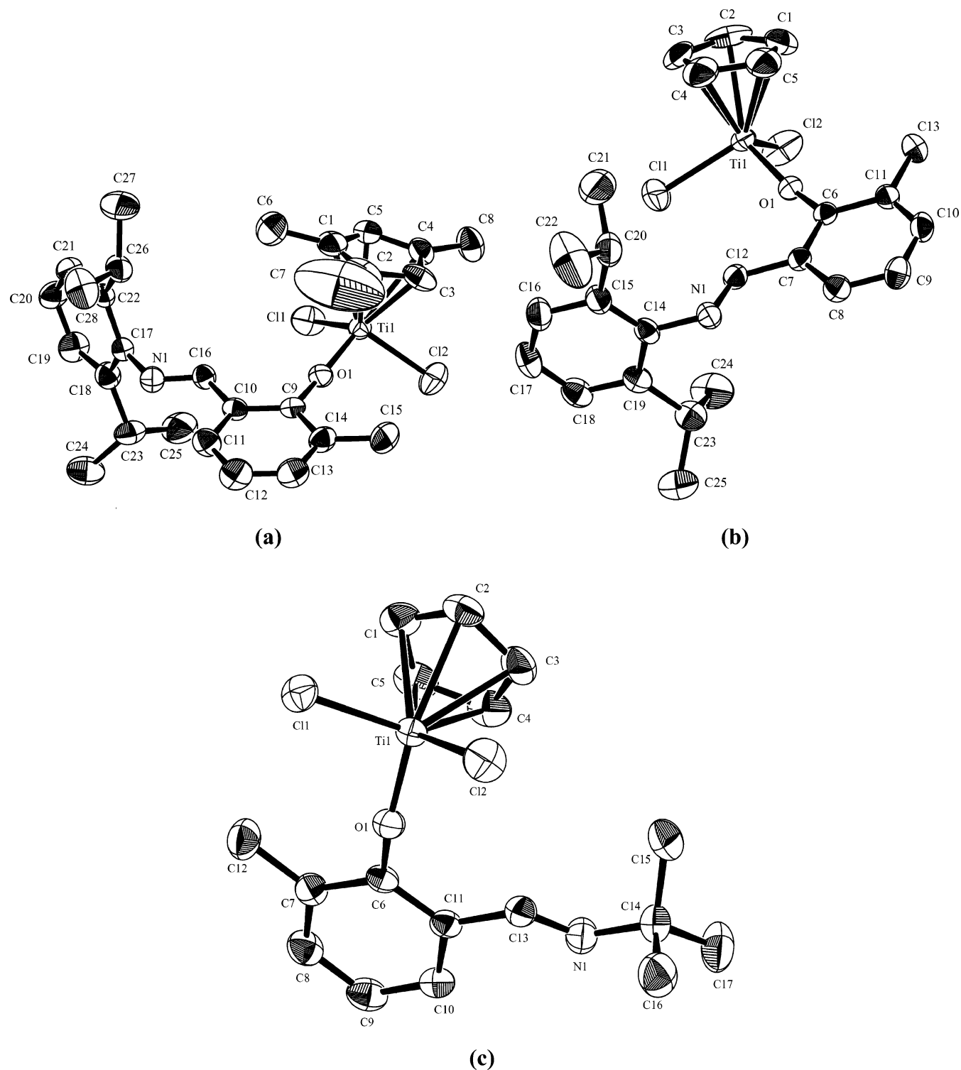
Figure 2. ORTEP drawings for \text{Cp}^*\text{TiCl}_2[\text{O}-2\text{-Me}-6\text{-(R}^2\text{N=CH)C}_6\text{H}_3] . \text{Cp}^* , \text{R}^2 = (a) 1,2,4- \text{Me}_3\text{C}_5\text{H}_2 , 2,6- ^i\text{Pr}_2\text{C}_6\text{H}_3 ( 5 ), (b) Cp, 2,6- ^i\text{Pr}_2\text{C}_6\text{H}_3 ( 6 ), (c) Cp, ^t\text{Bu} ( 7 ). Thermal ellipsoids are drawn at the 50% probability level and H atoms are omitted for clarity.
