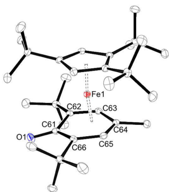
Figure 3. ORTEP diagram of 5-Me (ellipsoids at 50% probability level). Selected bond distances (Å) and angles (deg): Cp(cent)–Fe1 1.72, Fe1–Cp(plane) 1.717, Fe1–dienyl(plane) 1.635, Fe1–C61 2.4421(15), Fe1–C62 2.2098(14), Fe1–C63 2.1029(14), Fe1–C64 2.1221(16), Fe1–C65 2.0988(16), Fe1–C66 2.2115(16), C61–O1 1.2478(19), C61–C62 1.469(2), C62–C63 1.414(2), C63–C64 1.407(2), C64–C65 1.411(2), C61–C66 1.472(2), \angle Cp(plane)–dienyl(plane) 0.71.
