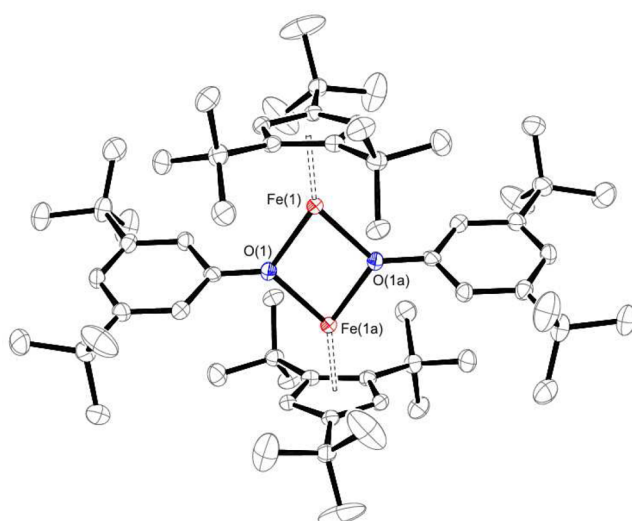
Figure 4. ORTEP diagram of 6 (ellipsoids at 50% probability level). Selected bond distances (Å) and angles (deg): Cp(cent)–Fe(1) 1.94, Fe(1)–O(1) 1.9881(12), Fe(1)–O(1a) 2.0115(13), Fe(1)···Fe(1a) 3.06, O(1)–Fe(1)–O(1a) 80.03(5), Fe(1)–O(1)–Fe(1a) 99.97(5).
