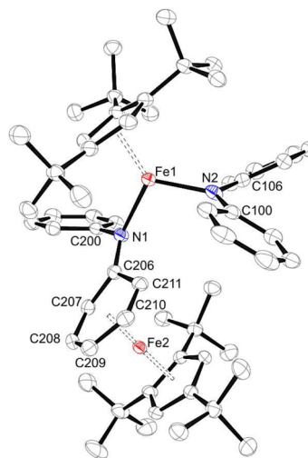
Figure 5. ORTEP diagram of 8 (ellipsoids at 50% probability level). Selected bond distances (Å) and angles (deg): \text{Cp}(\text{cent})\text{--Fe1} 2.04, \text{Cp}(\text{plane})\text{--Fe1} 2.036, \text{Cp}(\text{cent})\text{--Fe2} 1.68, \text{Cp}(\text{plane})\text{--Fe2} 1.683, \text{Fe1--N1} 2.1494(18), \text{N1--C200} 1.436(3), \text{N1--C206} 1.333(3), \text{Fe1--N2} 2.047(2), \text{N2--C100} 1.387(3), \text{N2--C106} 1.398(3), \text{C206--C207} 1.441(3), \text{C207--C208} 1.414(3), \text{C208--C209} 1.406(3), \text{C210--C211} 1.409(3), \text{C211--C206} 1.434(3), \text{Fe2--dienyl}(\text{plane}) 1.563, \text{Fe2--C206} 2.427(2), \text{Fe2--C207} 2.124(2), \text{Fe2--C208} 2.054(2), \text{Fe2--C209} 2.076(2), \text{Fe2--C210} 2.060(2), \text{Fe2--C211} 2.128(2), \angle \text{Cp}(\text{plane})\text{--dienyl}(\text{plane}) 1.89.
