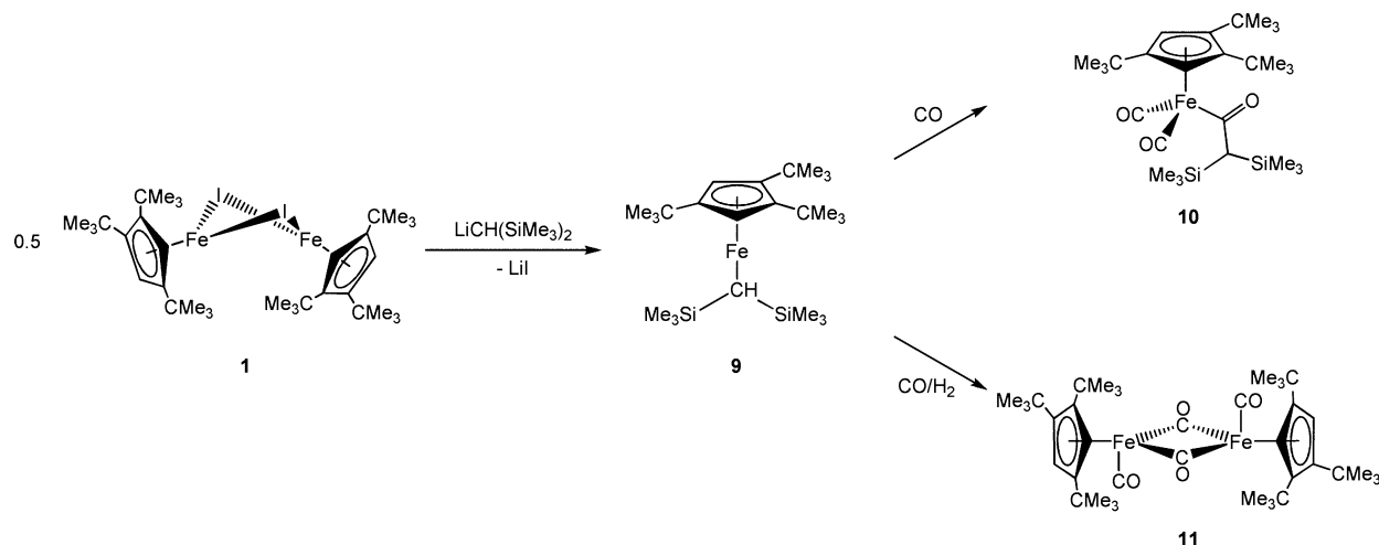
Scheme 6. Synthesis and Reactivity of 9
