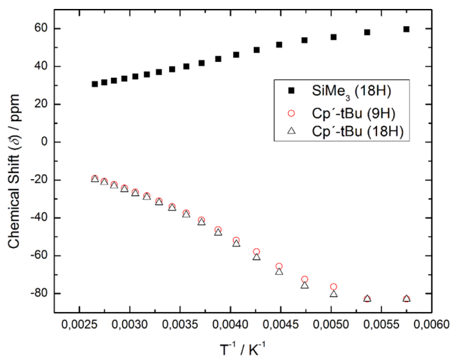
Figure 6. Chemical shift ( \delta ) vs T^{-1} plot for 7 .
