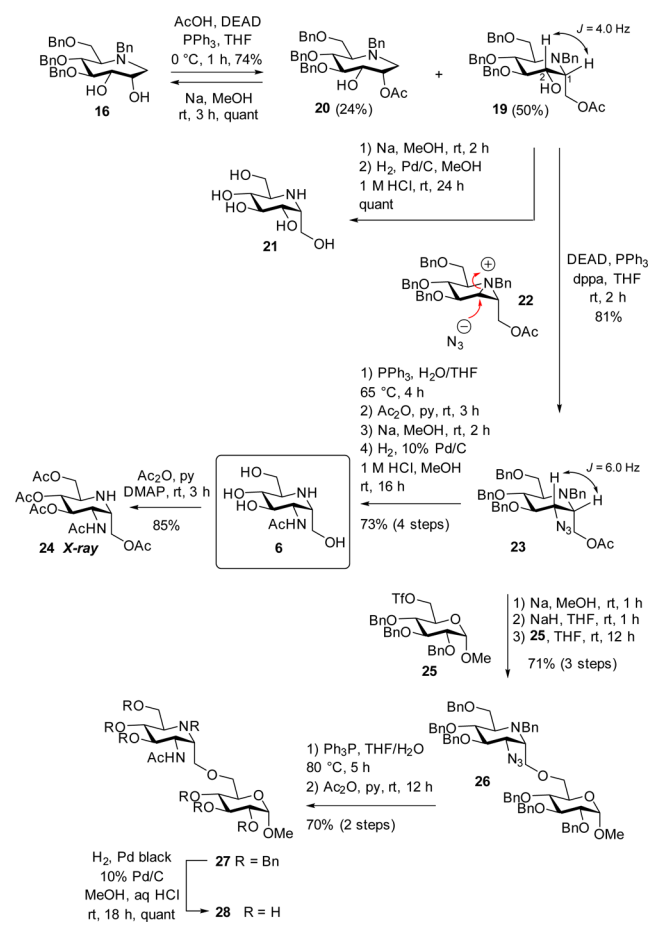
Scheme 3. Synthesis of \alpha -HNJNac 6 and Pseudodisaccharide 28
