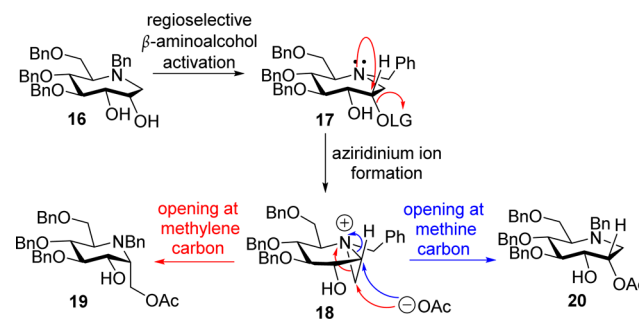
Scheme 2. Proposed Mechanism for the Ring Contraction of Azepane 16 Leading to Piperidine 19 and Azepane 20
