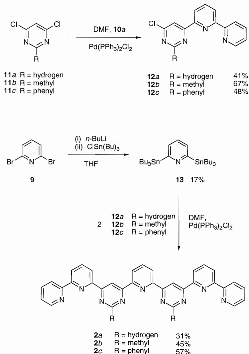
Fig. 5. Synthesis of tris-tridentate ligands 2a–c .
