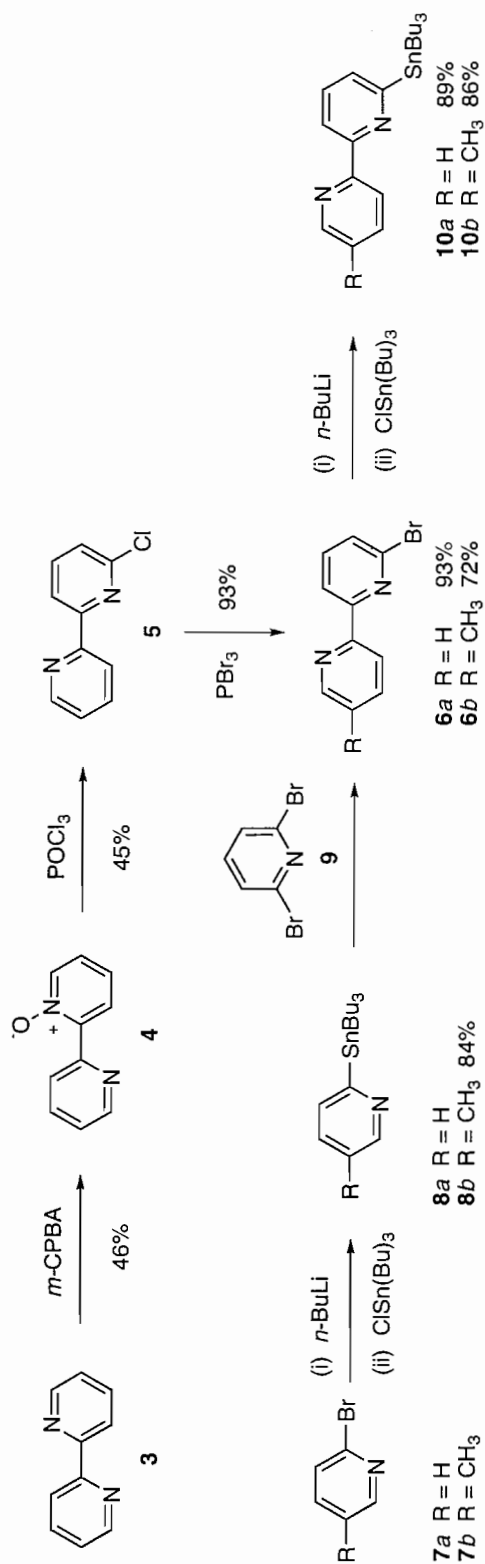
Fig. 3. Synthesis of 6-tributylstannyl-2,2'-bipyridines 10a,b from 2,2'-bipyridine and stannyl pyridines 8a,b .
