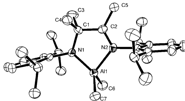
Figure 3. ORTEP plot of 11 at the 50% probability level. The hydrogen atoms have been omitted for clarity. Selected bond lengths (Å) and angles (deg): Al(1)–N(1) = 1.845(2) , Al(1)–C(7) = 1.961(3) , Al(1)–C(6) = 1.961(3) , Al(1)–N(2) = 1.980(2) , N(1)–C(1) = 1.477(3) , N(2)–C(2) = 1.303(4) , C(7)–Al(1)–C(6) = 108.21(15) , N(1)–Al(1)–N(2) = 84.59(10) .
