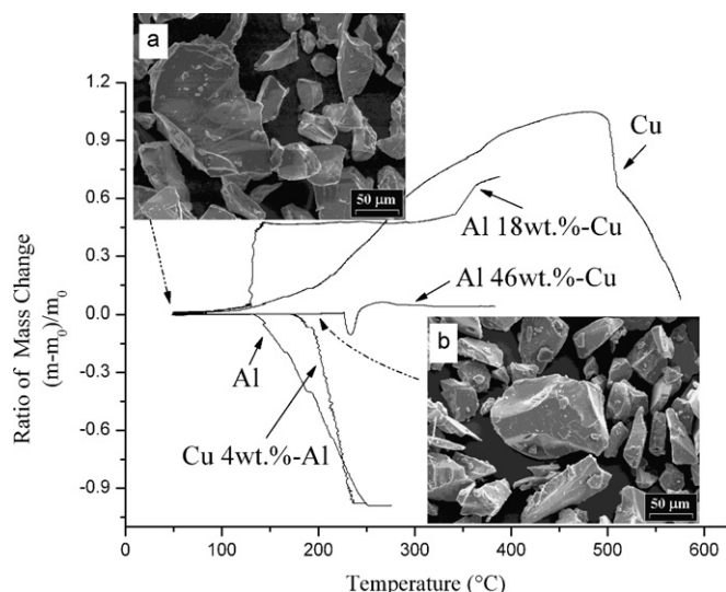
Fig. 2. Non-isothermal TG curves for the chlorination of Cu, Al, Al 18 wt.%-Cu, Al 46 wt.%-Cu, and Cu 4 wt.%-Al. (a) Initial sample for the chlorination of Al 46 wt.%-Cu, (b) unreacted Al 46 wt.%-Cu alloy after 2 h of chlorination at 200 °C.
