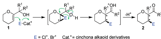
Scheme 2. Design for the Catalytic Enantioselective Halogenation/Semipinacol Rearrangement
