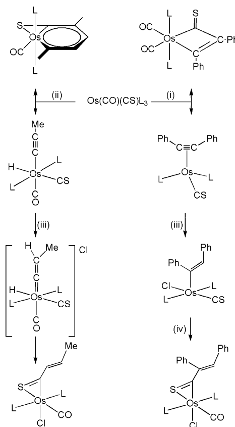
Scheme 2. Osmium Alkenyl–Thiocarbonyl Migratory Insertion Reactions (L = \text{PPh}_3 ) a,7b,f
