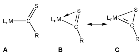
Chart 1. Thioacyl and Metallathiirene Canonical Forms
