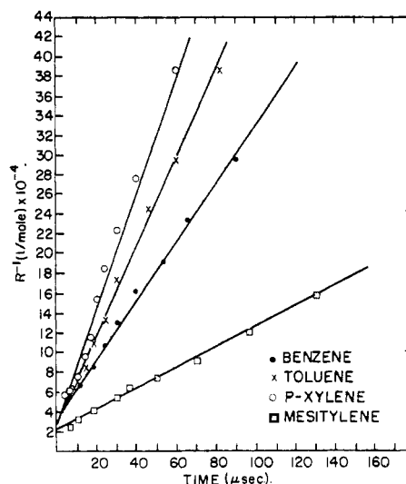
Fig. 3.—Plot of reciprocal radical concentration versus time for the aromatic hydrocarbon.
