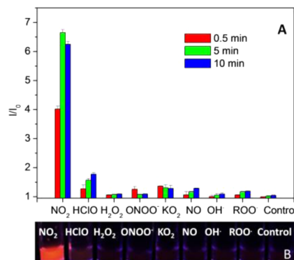
Figure 1. Ortho isomer 6 is selective toward common ROS under physiological conditions. (A) Fluorescence responses obtained upon addition of various ROS (1 \mu M) to 6 (0.2 \mu M) delivered using 20 equiv of DOTAP in 10 mM PBS (pH 7.4) at 37 °C ( \lambda_{\text{ex}} = 540 nm, \lambda_{\text{em}} = 590 nm). (B) Digital photos showing that NO 2 turns on the fluorescence but other ROS do not under illumination by a 365 nm UV lamp 5 min after addition of ROS (5 \mu M) to 6 (1 \mu M) delivered using 20 equiv of DOTAP in 10 mM PBS (pH 7.4).
