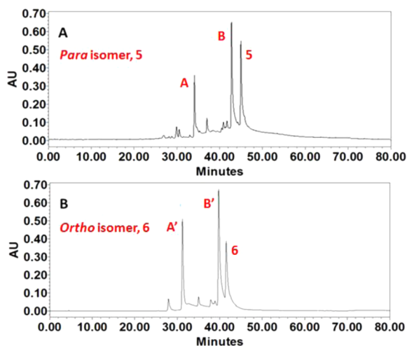
Figure 3. HPLC chromatograms of the products of the reactions of 5 and 6 with NO 2 , recorded at 560 nm.
