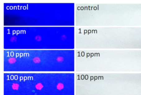
Figure 4. Visual detection of NO 2 gas. NO 2 concentrations of 0, 1, 10, and 100 ppm were tested. The images on the left were obtained under illumination by a 352 nm UV lamp in the dark. For comparison, no color can be seen in the images on the right, which were obtained under laboratory lighting without UV light excitation.
