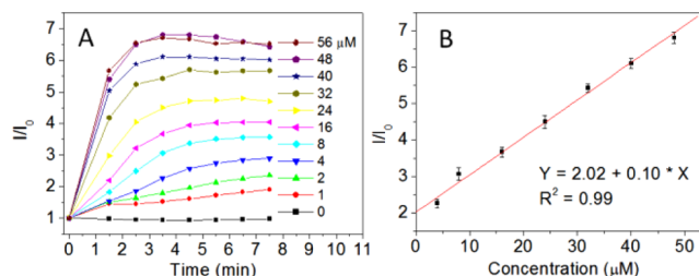
Figure 2. Responses of ortho isomer 6 to DEANO at different concentrations under physiological conditions. (A) Increments of fluorescence intensity of 6 (0.2 \mu M) delivered using 20 equiv of DOTAP against time after the addition of DEANO at different concentrations in 10 mM PBS (pH 7.4) at 37 °C ( \lambda_{\text{ex}} = 540 nm, \lambda_{\text{em}} = 590 nm). (B) Dose-response curve for the fluorescence intensity of 6 (0.2 \mu M) delivered using 20 equiv of DOTAP obtained 3.5 min after the addition of DEANO in 10 mM PBS (pH 7.4) at 37 °C ( \lambda_{\text{ex}} = 540 nm, \lambda_{\text{em}} = 590 nm).
