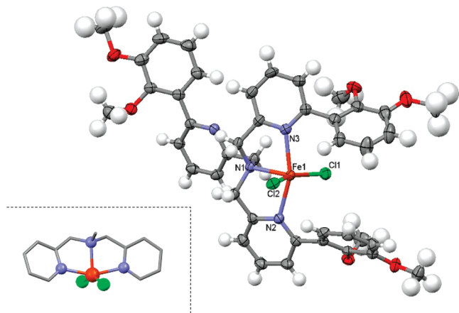
Figure 3. Mercury view of complex L_3FeCl_2 . Principal distances (in Å) and angles (in deg): FeN1, 2.183(2); FeN2, 2.235(2); FeN3, 2.205(2); FeCl1, 2.2930(8); FeCl2, 2.3576(7); N2FeN3, 156.89(8); N1FeCl1, 108.62 (6); N1FeCl2, 98.66(6); Cl2FeCl1, 152.61(3).
