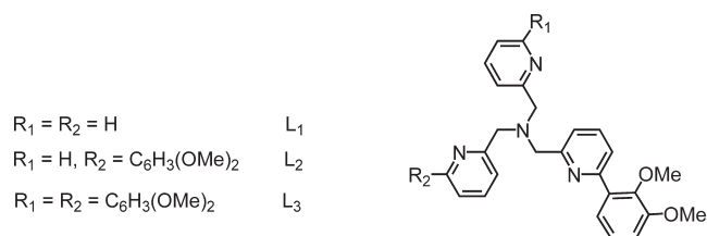
Figure 1. Ligands used in this study.
