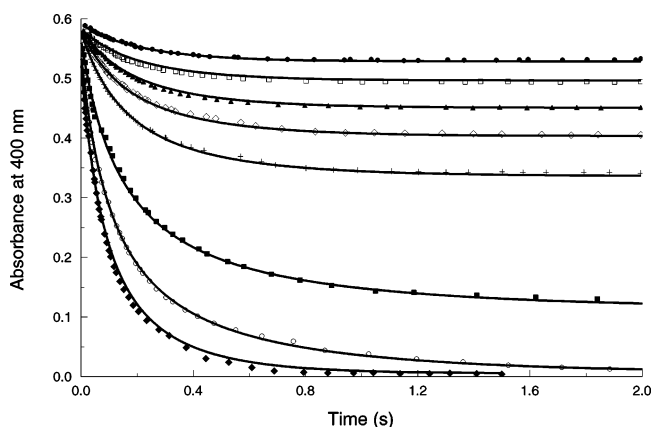
Figure 2. Measured (symbols) and calculated (solid lines) kinetic curves at pH = 3.65 and [\cdot\text{ClO}_2]_0 \approx 0.00075 \text{ M} . [\text{S(IV)}]_0 (\text{mM}) = 0.2 (\bullet), 0.3(\square), 0.5(\blacktriangle), 0.7(\diamond), 1.0(+), 2.0(\blacksquare), 3.0(\circ), 4.0(\blacklozenge) .
