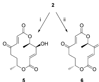
Scheme 2. Oxidation of Clonostachydiol ( 2 ): (i) Dess–Martin, (ii) \text{MnO}_2
