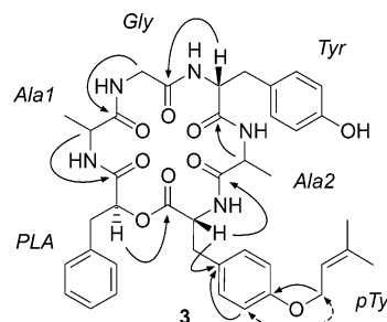
Figure 2. Long-range \text{H,C} -couplings (arrows) and one ROE interaction (dashed arrow) define the amino acid sequence of 3 and the position of the prenyl group.
