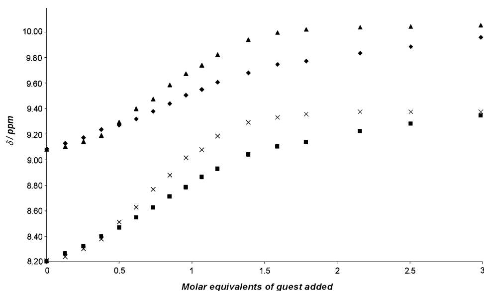
Figure 6. Binding titration curves for macrocycle 1 , showing the shift of a) the amide (◆: Ac-L-Glu, ▲: Ac-D-Glu) and b) the thiourea (■: Ac-L-Glu, ×: Ac-D-Glu) NH protons on addition of the bis(tetrabutylammonium) salts of N-Ac-L-glutamate and N-Ac-D-glutamate in CD 3 CN as solvent (1:1 [host]:[guest] is reached when [guest]=1.5 mM).
