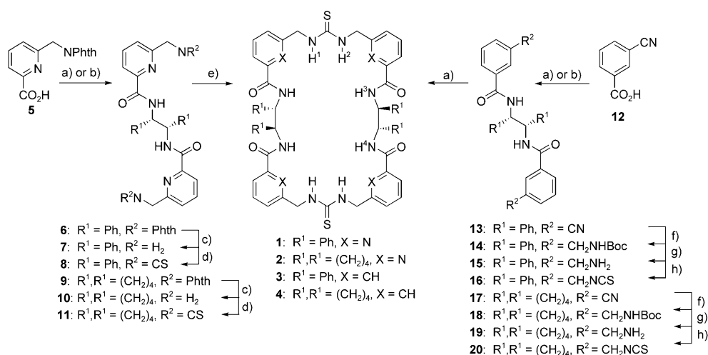
Scheme 1. a) SOCl 2 ; (1 S ,2 S )-(-)-1,2-diphenylethylenediamine, DMAP, CH 2 Cl 2 (68% for 6 , 48% for 13 ); b) diphenylchlorophosphate; (1 S ,2 S )-(-)-1,2-diaminocyclohexane (tartrate salt), H 2 O, K 2 CO 3 (52% for 9 , 67% for 17 ); c) N 2 H 4 ·H 2 O, EtOH (80–85%); d) CS 2 , DCC, CH 2 Cl 2 ; e) simultaneous addition of 1 equiv of 7 (or 10 or 15 or 19 ) and 1 equiv of 8 (or 11 or 16 or 20 , respectively) by syringe pumps over 3 h to a solution of DMAP or Et 3 N in CH 2 Cl 2 (26% for 1 , 72% for 2 , 17% for 3 , 29% for 4 , over steps d and e or h and e); f) di- tert -butyl dicarbonate, NiCl 2 , NaBH 4 (64% for 14 and 18 ); g) TFA, CH 2 Cl 2 (quant.); h) thiophosgene, K 2 CO 3 , CH 2 Cl 2 , H 2 O. DMAP = 4-dimethylaminopyridine, DCC = N,N' -dicyclohexylcarbodiimide, TFA = trifluoroacetic acid.
