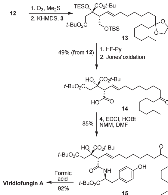
Scheme 3. Completion of Viridiofungin A
