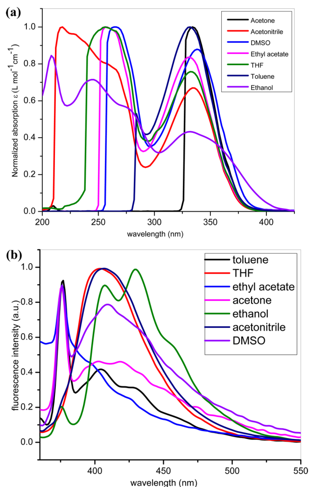
Figure 3. (a) UV-vis absorption spectra of 3q (10 \mu M) in different solvents, and (b) fluorescence emission spectra of 3q (10 \mu M) in different solvents.
