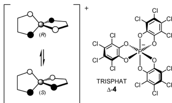
Figure 1. Stereodynamics among diastereoisomeric [\text{CuL}_2][\Delta\text{-4}] ion pairs.
