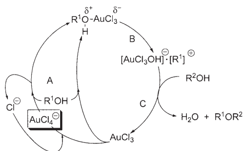
Scheme 3. Catalytic cycle.
