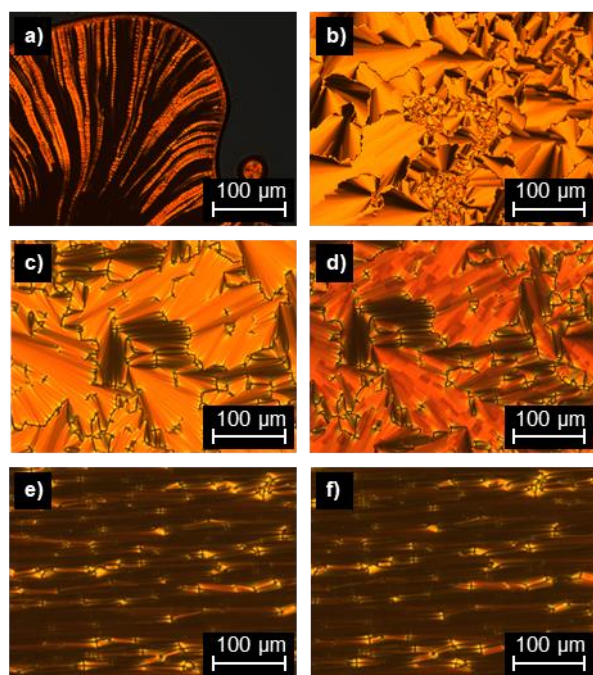
Figure 5 Polarized optical micrographs of a) 2-Fla-1 at 135^\circ\text{C} (magnification 100x) upon heating, b) 2-Fla-1 at 115^\circ\text{C} (magnification 100x) upon cooling from the isotropic liquid, c) fan-shaped textures at 135^\circ\text{C} and at d) 110^\circ\text{C} . 2-Fla-1 in a rubbed polyimide cell (homogeneous alignment, cell gap: 3 \mu\text{m} ) upon cooling. 2-Fla-1 in a single side rubbed nylon cell, cell gap: 1.6 \mu\text{m} ) at e) 135^\circ\text{C} and f) 110^\circ\text{C} .
