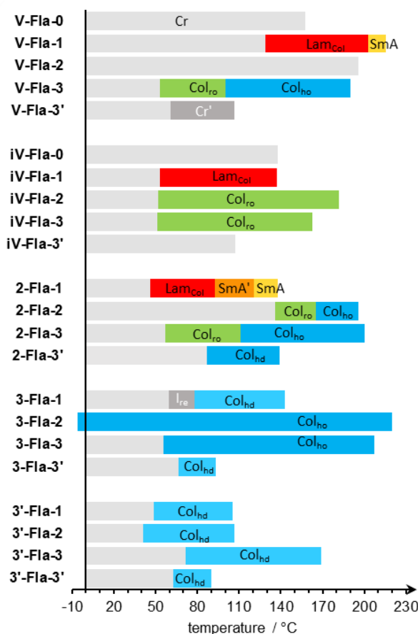
Figure 2 Overview of the observed mesophase of the flavylium salts A-Fla-B (a detailed version of this diagram with the mesophase width can be found in Figure S1).
