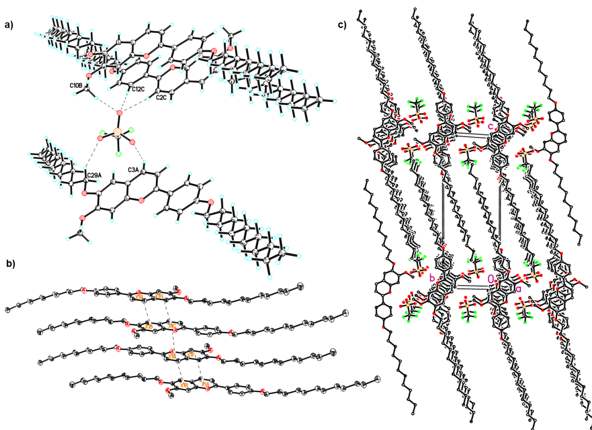
Figure 1 Single crystal X-ray structure representations of V-Fla-1 in the solid state [31] (H = light blue, C = white, O = red, S = yellow, F = green, in b) and c) hydrogens are omitted for clarity). a) Hydrogen bond interactions of the triflate anion given by dashed lines. b) Stacking interaction of the flavylium cation. c) bc view along the a -axis showing the interdigitated layer structure.
