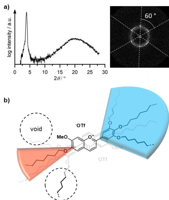
Figure 11 a) WAXS diffractogram of 3-Fla-1 at 85 °C. The inset displays the SAXS pattern of a planar aligned domain obtained by slow heating into the Col h phase at 80 °C (the additional diffuse reflex is most likely due passing of the beam through another domain without mesophase). b) Proposed stacking of two flavylum cations V-Fla-3 in the liquid crystalline state.
