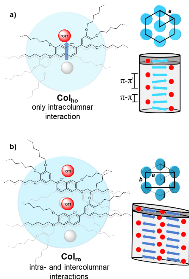
Figure 10 Proposed packing model of the flavylum salts in the a) \text{Col}_{\text{ho}} and the b) \text{Col}_{\text{ro}} mesophase viewed from the top (left) and in an side view (right).The flavylum
