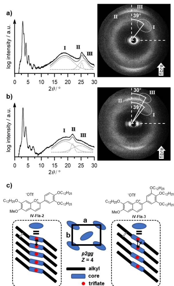
Figure 8 X-ray diffractograms of a fibre sample of a) iV-Fla-2 at 110 °C and b) iV-Fla-3 at 120 °C with the corresponding 2D diffraction pattern with the azimuthal angles of the diffuse wide-angle reflexes. The fitting of the wide-angle area is given in grey with the sum (bold line) of the distinct Gauss peaks (dashed lines). White arrows indicate the direction of the fibre. c) Proposed packing model of the Col ro phase and the stacking within the column (the representation of the discoid has been simplified, for a more detailed discussion see Figure 10 and the corresponding text).
