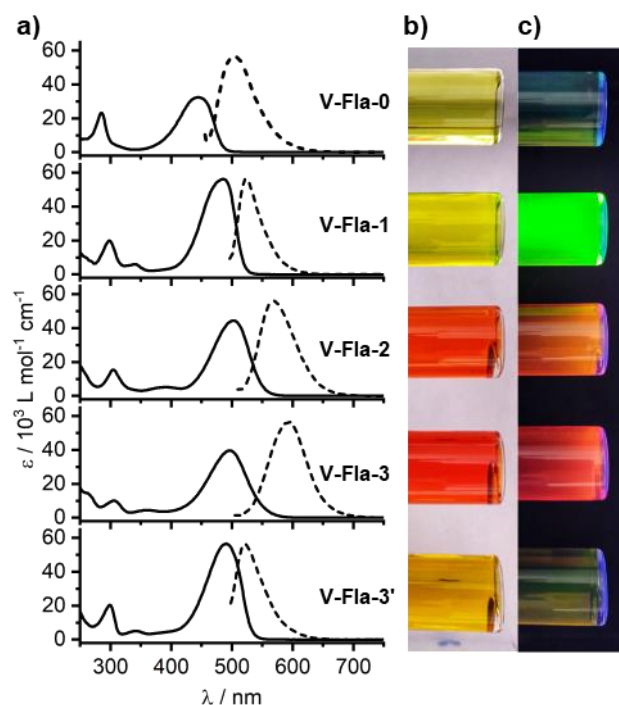
Figure 12 a) Absorption spectra (bold line, represented by its extinction coefficient determined by linear regression of a concentration series ranging from 0.2 \cdot 10^{-5} M to 7 \cdot 10^{-5} M) and normalized emission spectra (dashed line) of vanillin-derived flavylum salts V-Fla-B in \text{CHCl}_3 .
