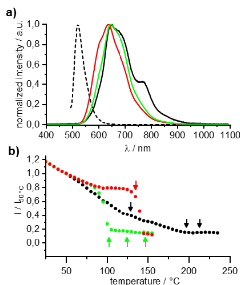
Figure 13 a) Emission spectra of V-Fla-1 (black), iV-Fla-1 (red) and 2-Fla-1 (green) in the solid state at 50 °C under irradiation with UV light (350 – 380 nm, solution spectra of V-Fla-1 is given in dashed lines for comparison) and b) temperature dependent emission intensity at 665 nm upon cooling the sample from the isotropic liquid (cooling rate of 10 K min -1 ). For the orientation transition temperatures of the DSC are given as arrows.
