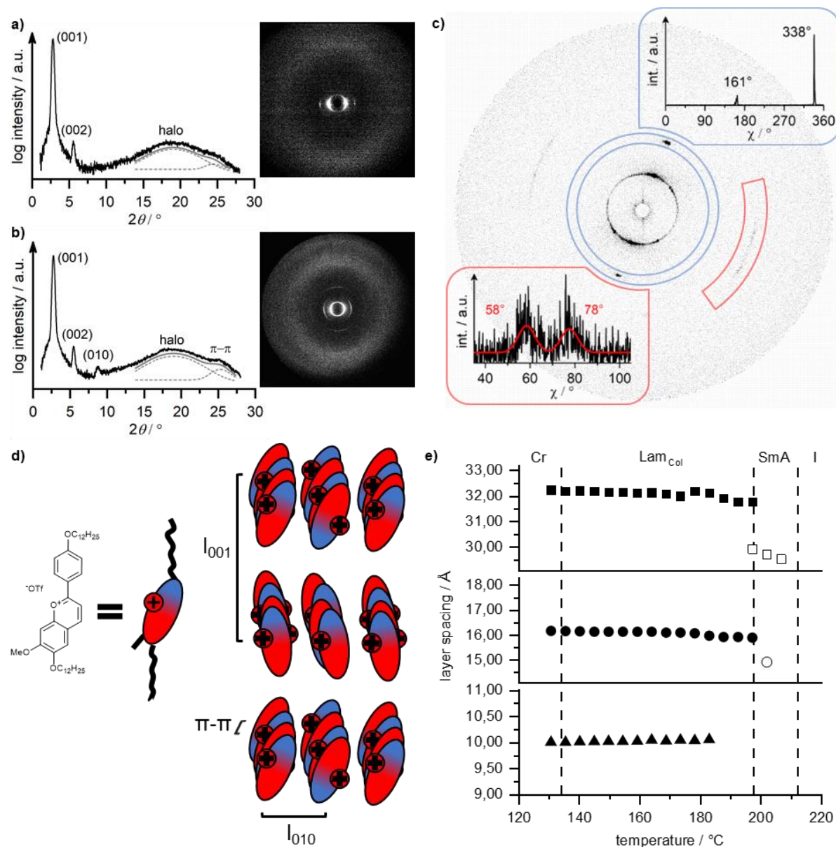
Figure 4 Diffractogram and the diffraction pattern of the oriented sample of V-Fla-1 in the a) SmA phase at 210 °C and b) LamCol phase at 170 °C after cooling from the isotropic state (cooling rate: 5 K min -1 ). c) 2D-SAXS pattern of the LamCol mesophase and the \chi -scan of the diffraction peaks obtained by slow cooling (0.2 K min -1 ) from the SmA phase into the LamCol phase. d) Proposed packing of the molecules in the LamCol mesophase. e) Temperature dependent layer spacing of the (001) reflex (■), the (002) reflex (●) and the (010) reflex (▲) in the SmA (hollow symbols) and the LamCol phase (filled symbols) of compound V-Fla-1 . The measurement was performed via the second heating (rate: 2 K min -1 ).
