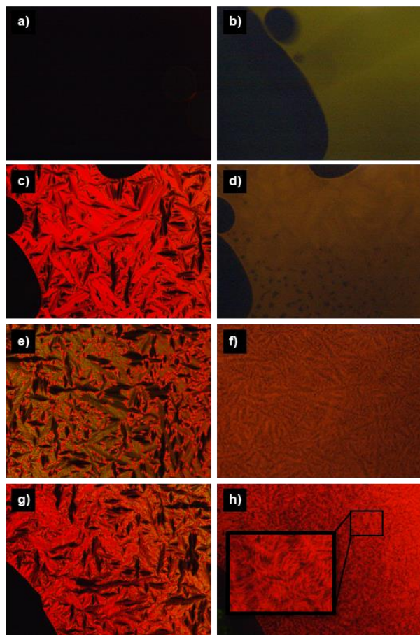
Figure 14 Optical micrographs of V-Fla-1 observed between crossed polarizers (left column) and under UV radiation (right column, without polarizer, exposure time: 8 seconds, the brightness of b) and d) has been increased by 40 % in order to ensure visibility) in the a-b) isotropic phase at 230 °C, c-d) the SmA phase at 200 °C, e-f) the LamCol phase at 170 °C and g-h) the crystalline phase at 30 °C. The images were obtained by cooling of the isotropic liquid with a cooling rate of 10 K min -1 .
