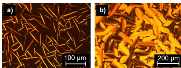
Figure 3 POM micrographs of a) V-Fla-1 at 205 °C (magnification 200x) and b) at 188 °C (magnification 100x). All pictures were taken between crossed polarizers upon cooling from the isotropic phase with a cooling rate of 5 K min -1 .
