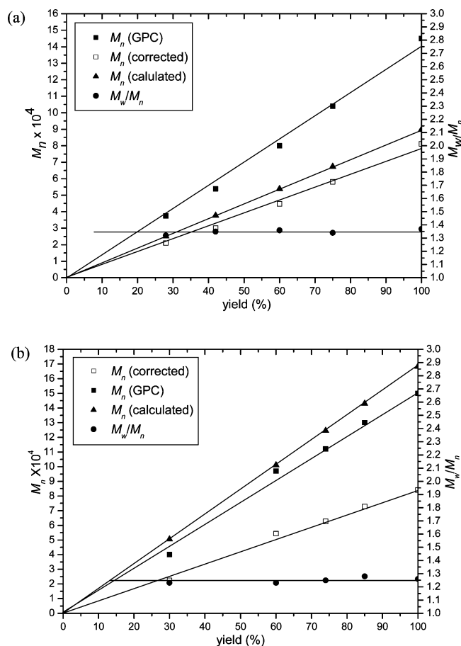
Figure 5. M n and M w / M n vs conversion plots for poly( \epsilon -CL) obtained using complexes 1 (a) and 2 (b). Conditions: [M] 0 /[I] 0 = 800, toluene, rt (for complex 1 ); [M] 0 /[I] 0 = 1500, toluene, 40 °C (for complex 2 ).
