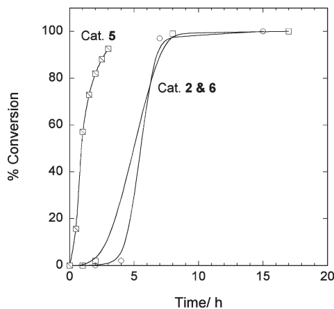
Figure 6. Reaction progress for the hydrosilylation of acetophenone with \text{PhSiH}_3 at 110 °C catalyzed by dioxomolybdenum(VI) 2 (open circles), dinuclear molybdenum(V) 6 (open squares), and oxomolybdenum(IV) 5 (hatched squares). % Conversion was determined by ^1\text{H} NMR. The lines are a smoothing function and not a kinetic fit.
