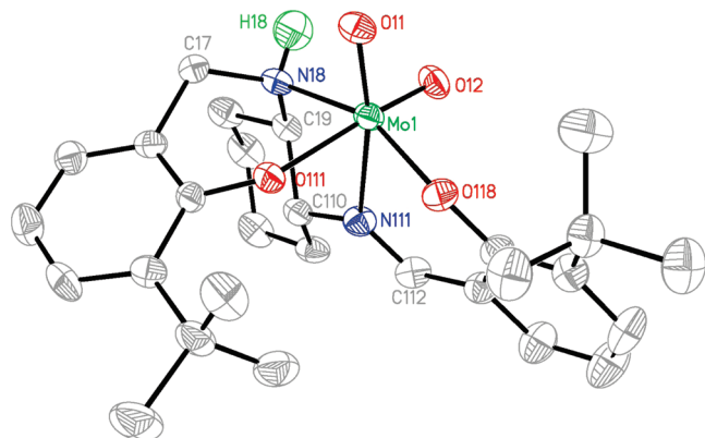
Figure 3. ORTEP diagram (drawn at 50% probability ellipsoids) of \text{Mo}(\text{O})_2(\text{saladach-}^t\text{Bu}) compound 2 . The hydrogen atoms except the one on nitrogen are omitted for clarity. Selected bond distances (Å) and bond angles (deg): \text{Mo1}-\text{O12} , 1.702(3); \text{Mo1}-\text{O11} , 1.712(2); \text{Mo1}-\text{O118} , 1.924(3); \text{Mo1}-\text{O111} , 2.016(2); \text{Mo1}-\text{N18} , 2.200(3); \text{Mo1}-\text{N111} , 2.297(3); \text{N111}-\text{C112} , 1.277(5); \text{N18}-\text{C17} , 1.501(4); \text{N18}-\text{H18} , 0.99(4); \text{N28}-\text{H28} , 0.71(4); \text{O12}-\text{Mo1}-\text{O111} , 160.20(12); \text{O118}-\text{Mo1}-\text{N18} , 155.79(12); \text{O11}-\text{Mo1}-\text{N111} , 169.51(12); \text{O12}-\text{Mo1}-\text{O11} , 101.59(12); \text{O12}-\text{Mo1}-\text{O118} , 100.87(13).
