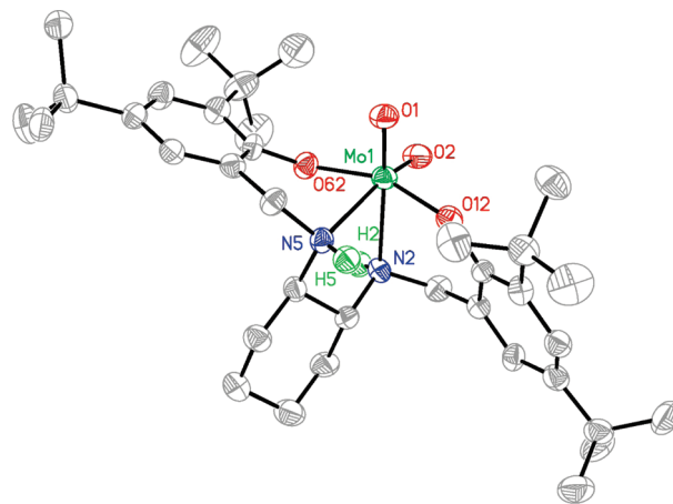
Figure 4. ORTEP diagram (drawn at 50% probability ellipsoids) of \text{Mo}(\text{O})_2(\text{salan-3,5-}^t\text{Bu}_2) compound 4 . The hydrogen atoms except the one on nitrogen are omitted for clarity. Selected bond distances (Å) and bond angles (deg): \text{Mo1}-\text{O2} , 1.688(4); \text{Mo1}-\text{O1} , 1.709(4); \text{Mo1}-\text{O12} , 1.924(4); \text{Mo1}-\text{O62} , 1.941(4); \text{Mo1}-\text{N2} , 2.347(5); \text{Mo1}-\text{N5} , 2.351(5); \text{O2}-\text{Mo1}-\text{O1} , 107.6(2); \text{O2}-\text{Mo1}-\text{O12} , 101.9(2); \text{O1}-\text{Mo1}-\text{O12} , 93.82(19); \text{O2}-\text{Mo1}-\text{O62} , 94.3(2); \text{O1}-\text{Mo1}-\text{O62} , 96.43(19); \text{O12}-\text{Mo1}-\text{O62} , 157.24(17); \text{O2}-\text{Mo1}-\text{N2} , 86.55(19); \text{O1}-\text{Mo1}-\text{N2} , 165.3(2); \text{O12}-\text{Mo1}-\text{N2} , 78.82(17); \text{O62}-\text{Mo1}-\text{N2} , 86.38(18); \text{O2}-\text{Mo1}-\text{N5} , 156.93(19); \text{O1}-\text{Mo1}-\text{N5} , 94.51(19); \text{O12}-\text{Mo1}-\text{N5} , 82.70(18); \text{O62}-\text{Mo1}-\text{N5} , 76.29(17); \text{N2}-\text{Mo1}-\text{N5} , 72.03(16).
