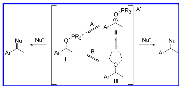
Figure 2. Possible modes of racemization.
