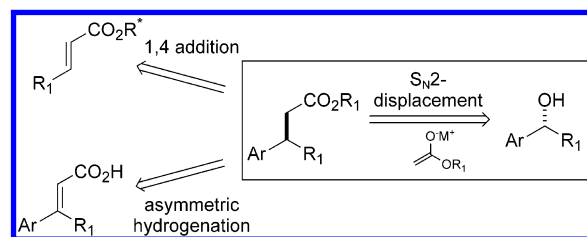
Figure 1. Approaches to 3-aryl-3-substituted propanoic acids.
