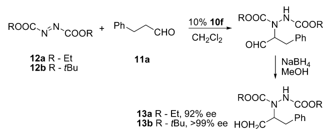
Scheme 10. Model Aminations Using 10f as the Organocatalyst
