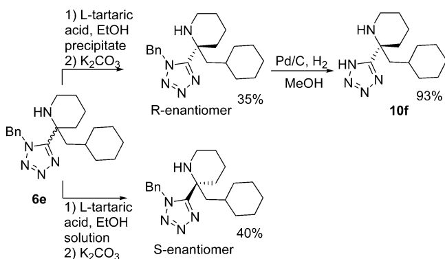
Scheme 9. Resolution of 6e into Enantiomers
