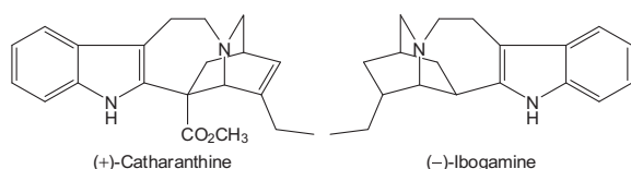
Figure 1. Iboga alkaloids.
