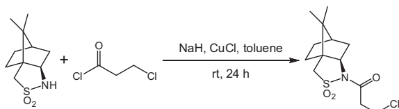
Scheme 2. Preparation of N -3-chloropropanoyl (1 S )-2,10-camphorsultam.
