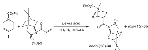
Scheme 1. Cycloaddition reaction of 1-phenoxy carbonyl-1,2-dihydropyridine 1 with N -acryloyl (1 S )-2,10-camphorsultam 2 in the presence of Lewis acid.
