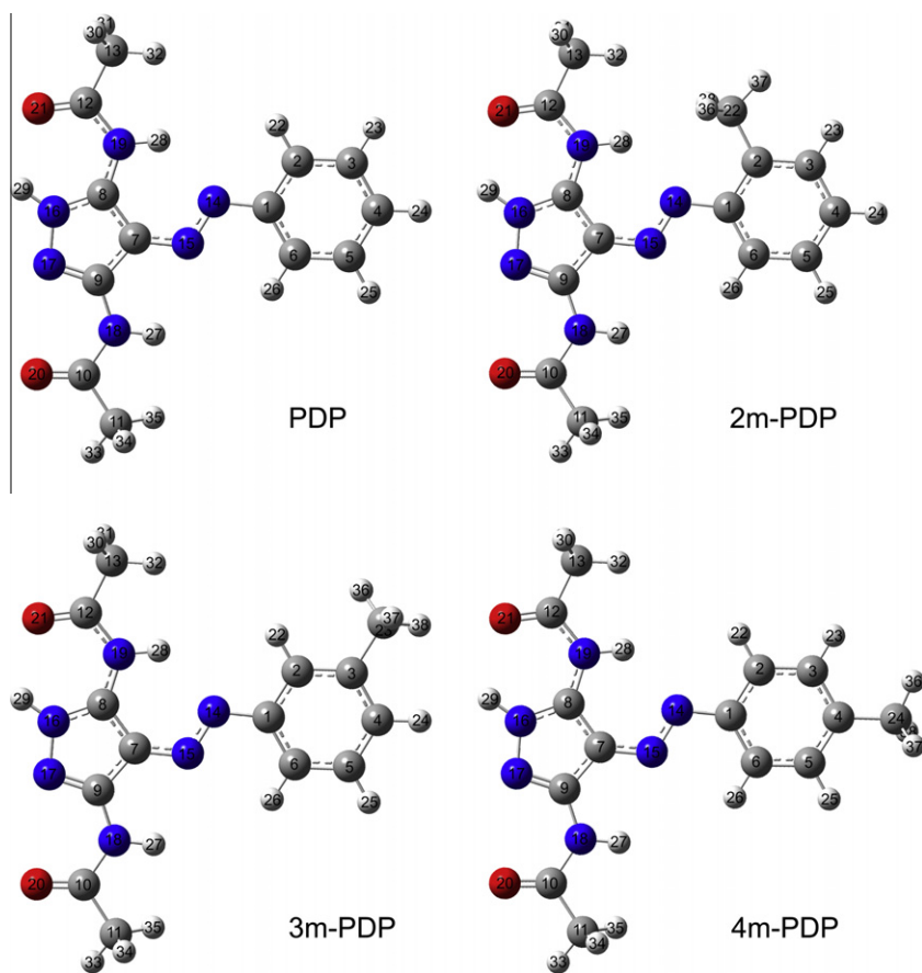
Fig. 1. The calculated optimized structures of 4-(substituted phenylazo)-3,5-diacetamido-1H-pyrazoles.
