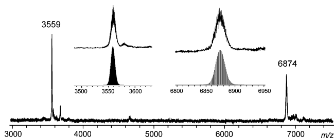
Figure 2. Positive-ion ESI-MS spectra of TBA 6 Nd-POM in acetone. Insets: spectra in the range of m/z 3490–3640 and 6800–6950 and simulated patterns for [TBA 6 H 4 Nd 2 (SiW 10 O 36 ) 2 ] 2+ ( m/z 3559) and [TBA 6 H 4 Nd 2 (SiW 10 O 36 ) 2 ] + ( m/z 6874).
