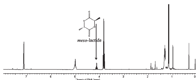
Figure 6. ^1\text{H} NMR spectrum in \text{C}_6\text{D}_6 during the ROP of L-lactide in the presence of complex 6d at ambient temperature. Methine proton of meso -lactide observed at 4.15 ppm.
