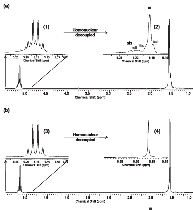
Figure 7. ^1\text{H} NMR spectra of poly(lactide) in \text{CDCl}_3 prepared from L-lactide. (a) In the presence of complex 6d , with 1 \rightarrow 2 illustrating expanded methine region before and after homonuclear decoupling. (b) In the presence of complex 6a , with 3 \rightarrow 4 illustrating expanded methine region before and after homonuclear decoupling.
