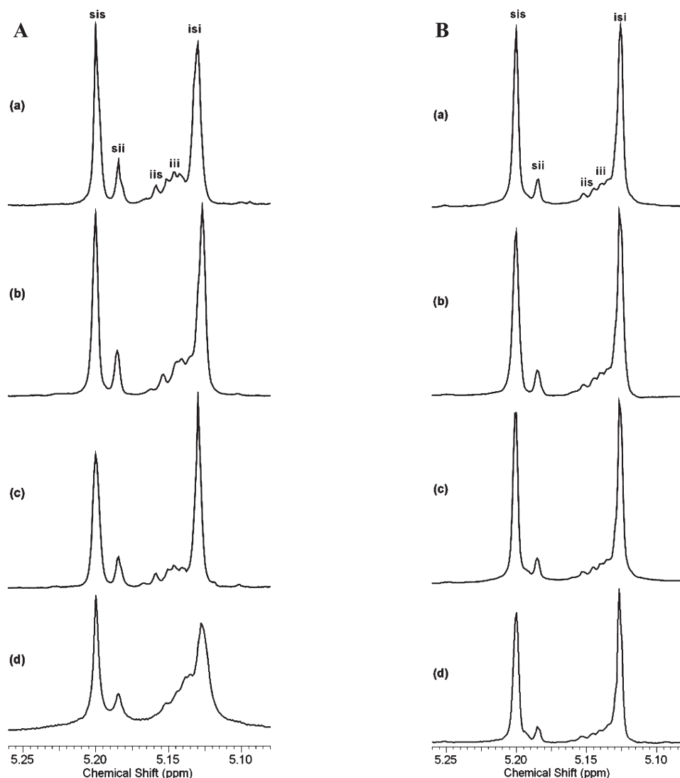
Figure 9. Homonuclear decoupled ^1\text{H} NMR ( \text{CDCl}_3 , 500 \text{MHz} ) spectra of the methine region of polylactide produced from rac -lactide with catalyst (a) 6a , (b) 6b , (c) 6c , and (d) 6d . (A) Polymerization temperature ambient. (B) Polymerization temperature -30\text{ }^\circ\text{C} .
