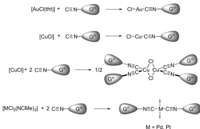
Scheme 3. Schematic representation of the various dendritic complexes prepared.
