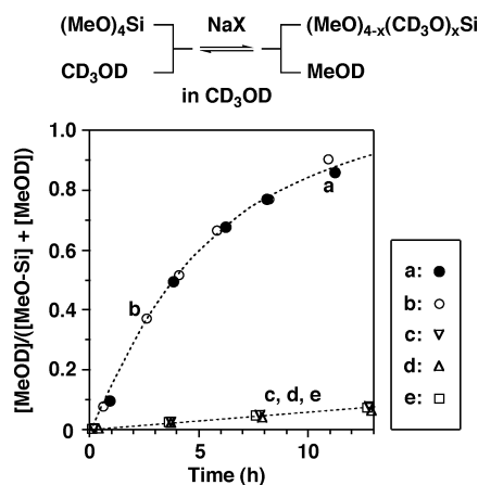
Figure 1. Time-courses of methoxy group exchanges between TMOS (initial concentration = 0.2 M) and \text{CD}_3\text{OD} in the absence (e) and presence of NaX (X = \text{BF}_4 (a), F (b), Br (c), and \text{NO}_3 (d)) at [\text{NaX}]_0/[\text{TMOS}]_0 = 6:100 in \text{CD}_3\text{OD} at 25^\circ\text{C} .
