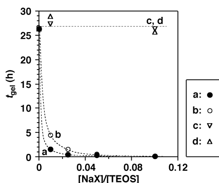
Figure 2. Hydrolytic condensation of TEOS at 25^\circ\text{C} in ethanolic aqueous HCl in the presence of \text{NaBF}_4 (a), NaF (b), NaBr (c), and \text{NaNO}_3 (d) at [\text{TEOS}]_0/[\text{H}_2\text{O}]_0/[\text{HCl}]_0/[\text{EtOH}]_0 = 1.0:23:1.0:3.5 . Times required to lose fluidity by gelation ( t_{\text{gel}} ).
