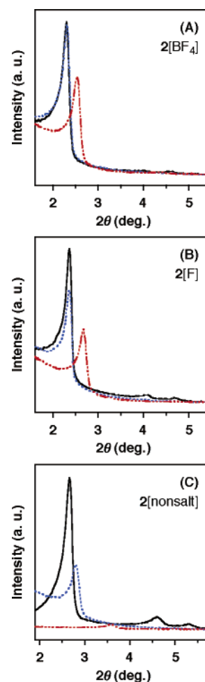
Figure 6. XRD patterns of calcined materials (A) 2[\text{BF}_4] , (B) 2[\text{F}] , and (C) 2[\text{nonsalt}] before (solid black curves) and after being heated in air at 900 °C for 3 h (broken red curves) or in water at 100 °C for 32 h (broken blue curves).
