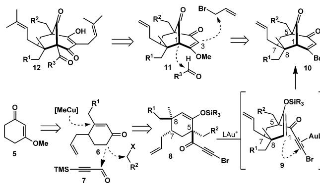
Scheme 1. Retrosynthetic analysis.
