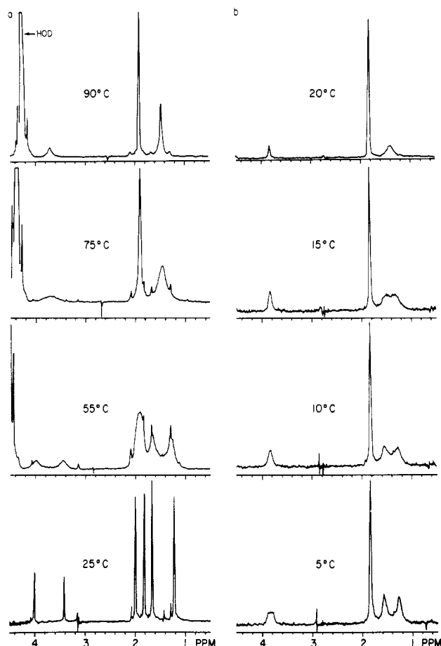
Figure 2. Variable-temperature ^1\text{H} NMR spectra of (a) [(\text{D-pen})-(\text{L-pen})\text{ReO}]^- ( 2b ) and (b) [(\text{D-pen})-(\text{L-pen})\text{TcO}]^- ( 2a ) in \text{D}_2\text{O} . Sharp resonances in the rhenium spectra are due to small amounts of 1b , which form slowly at elevated temperatures in solutions of 2b . 8
