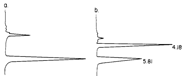
Figure 1. Reversed-phase HPLC traces of the products formed when ^{99}\text{TcO}_4^- was reduced in the presence of (a) D-penicillamine and (b) racemic penicillamine. Complex 1a is at 5.81 min and 2a is at 4.18 min. See Experimental Section for chromatographic conditions.
