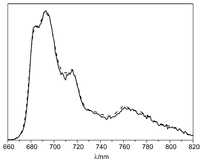
Figure 6. Steady-state emission spectrum (—) and the time-gated (10 \mu s–1.3 ms) emission spectrum (---) of AuP in EPA at 80 K. The excitation wavelength was 518 nm.
