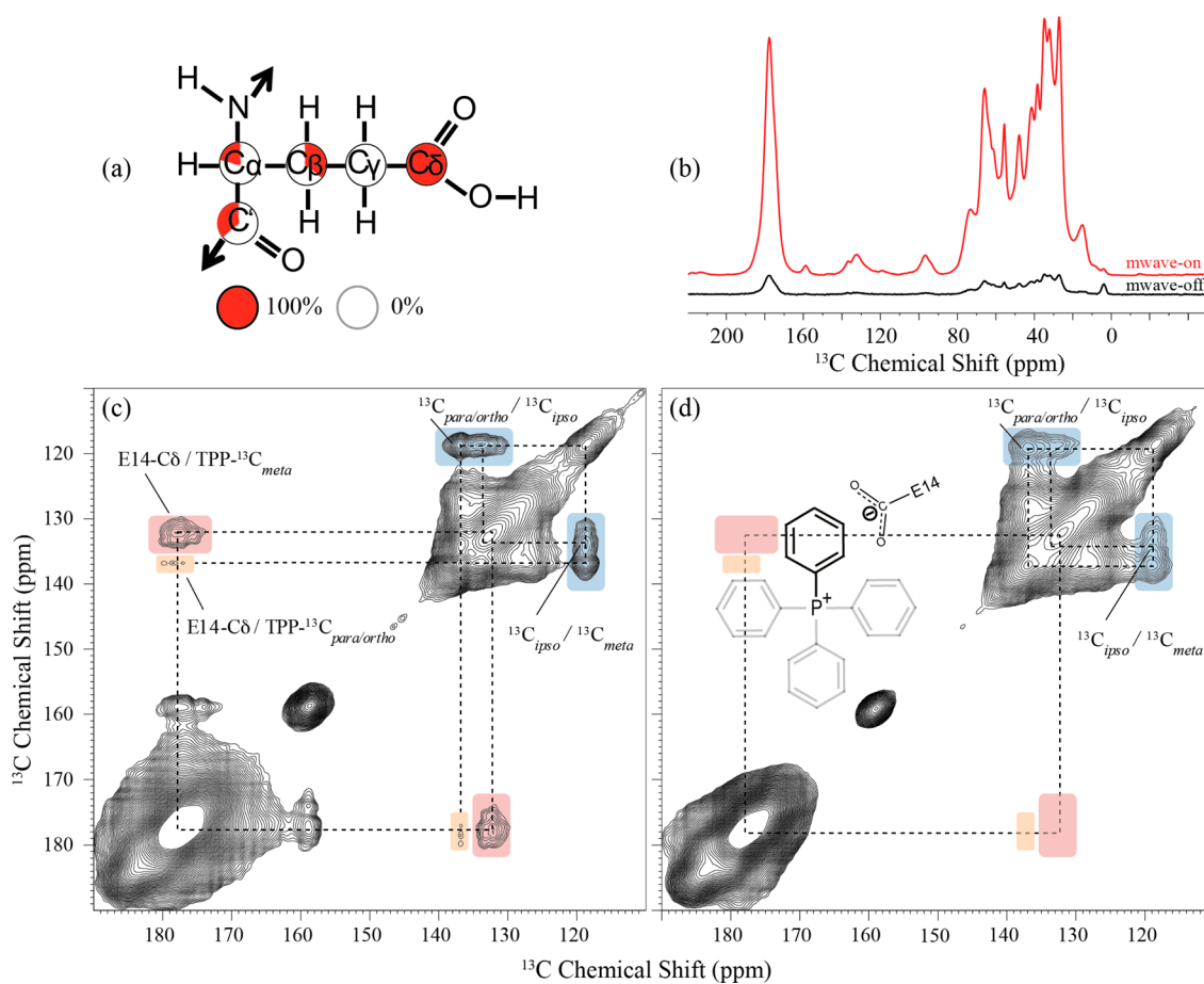
Figure 4. DNP-enhanced ^{13}\text{C} – ^{13}\text{C} DARR spectrum of ^{13}\text{C} -labeled EmrE in complex with ^{13}\text{C} -TPP ^{+} . EmrE was labeled using 2- ^{13}\text{C} -glycerol as sole carbon source, resulting in a sparse isotope distribution in which C \delta of glutamate is 100% ^{13}\text{C} -enriched (a). In these samples, labeling of aromatic amino acids was suppressed to avoid signal overlap with ^{13}\text{C} -TPP ^{+} ( ^{13}\text{C} -EmrE _1 ). For DNP, samples were doped with 20 mM TOTAPOL resulting at 100 K in a 19-fold signal enhancement (b). Both spectra were recorded with 32 scans. A ^{13}\text{C} – ^{13}\text{C} DARR spectrum (300 ms mixing time) reveals specific through-space correlations between ^{13}\text{C} -EmrE _1 and ^{13}\text{C} -TPP ^{+} (c), which are not observed when labeling of glutamates is suppressed ( ^{13}\text{C} -EmrE _2 ) (d). The observed correlation therefore arises from a direct interaction between ^{13}\text{C} -TPP ^{+} and the side chain of E14 (see text for further details), and our data indicate a defined orientation of TPP ^{+} with respect to the E14 side chain.
