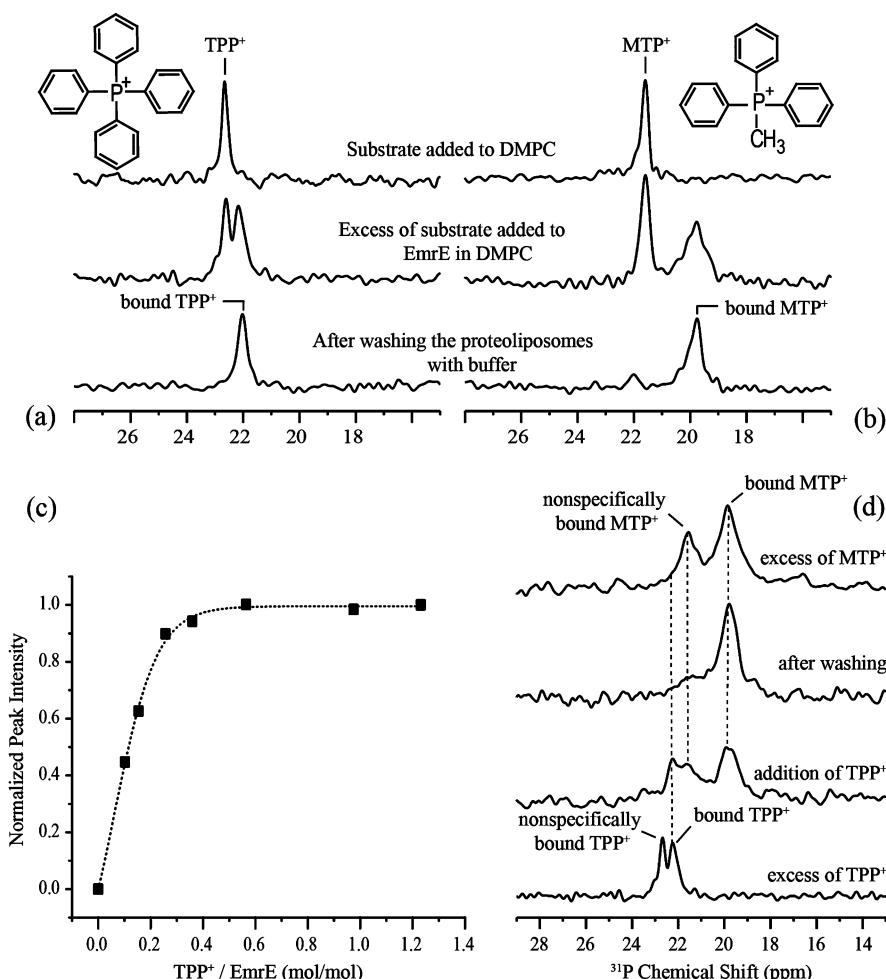
Figure 2. Detection of TPP ^{+} (a) and MTP ^{+} (b) specifically bound to EmrE observed by ^{31}\text{P} MAS NMR. Adding TPP ^{+} and MTP ^{+} to DMPC liposomes results in signals at 22.8 ppm (TPP ^{+} ) and 21.3 ppm (MTP ^{+} ) (top row). Adding excess substrate to EmrE reconstituted into DMPC results in two TPP ^{+} populations at 22.3 and 22.7 ppm and two MTP ^{+} peaks at 19.7 and 21.5 ppm (middle row). A molar ratio of two substrates per EmrE dimer was used. The low-field populations show almost identical chemical shifts to those observed in the absence of EmrE and disappear upon sample washing (bottom row). They correspond to free and nonspecifically bound ligands, while the remaining high-field signals result from specifically bound substrates. The latter show slightly smaller chemical shifts (TPP ^{+} , 22.1 ppm; MTP ^{+} , 19.3 ppm) and more narrow lines. Upon TPP ^{+} titration, the intensity of the signal from the specifically bound population saturates above a molar ratio of 2 EmrE/1 TPP ^{+} (c). Competitive titration experiments show that TPP ^{+} displaces MTP ^{+} bound to EmrE (d). All spectra were acquired using ^1\text{H} – ^{31}\text{P} cross-polarization except for TPP ^{+} /MTP ^{+} in pure DMPC bilayers, which were recorded using direct polarization.
