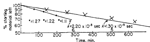
Figure 1. Log plot of per cent decomposition of 5 and 6 at 152.0°: X, per cent 5 left; ●, per cent 6 left; *, 5/9 + 10 from 6 ; k in \text{sec}^{-1} .
