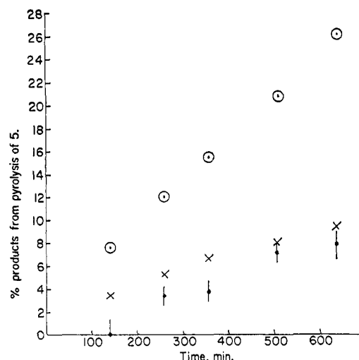
Figure 2. Per cent of products from pyrolysis of 5 as a function of time at 152.0°: ○, per cent of 9 + 10 ; X, per cent of 6 ; ↑, per cent racemization of 5 .
