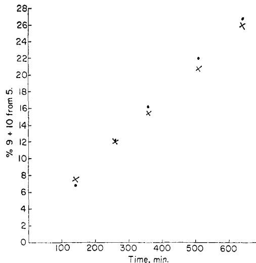
Figure 5. Per cent 9 + 10 from active 5 as a function of time at 152.0°C: ×, experimental; ●, calcd with k_2 = 0.13 \times 10^{-5} \text{ sec}^{-1} .
