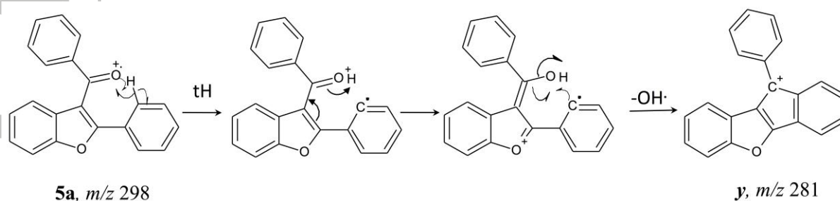
Scheme 4. Proposed mechanism of OH. loss for 5a
