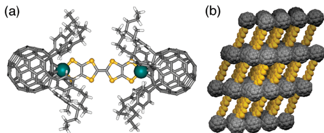
Figure 1. X-ray crystal structure of 4\bullet(\text{CS}_2)\bullet(\text{C}_6\text{H}_6) . Solvent molecules are omitted for clarity. (a) Ball and stick drawing. Location of the carbon atoms in the butyl chains were optimized with geometrical restraints on the SHELX97 program. 23 (b) CPK drawing of the crystal packing. The butyl phenyl groups are omitted for clarity.
