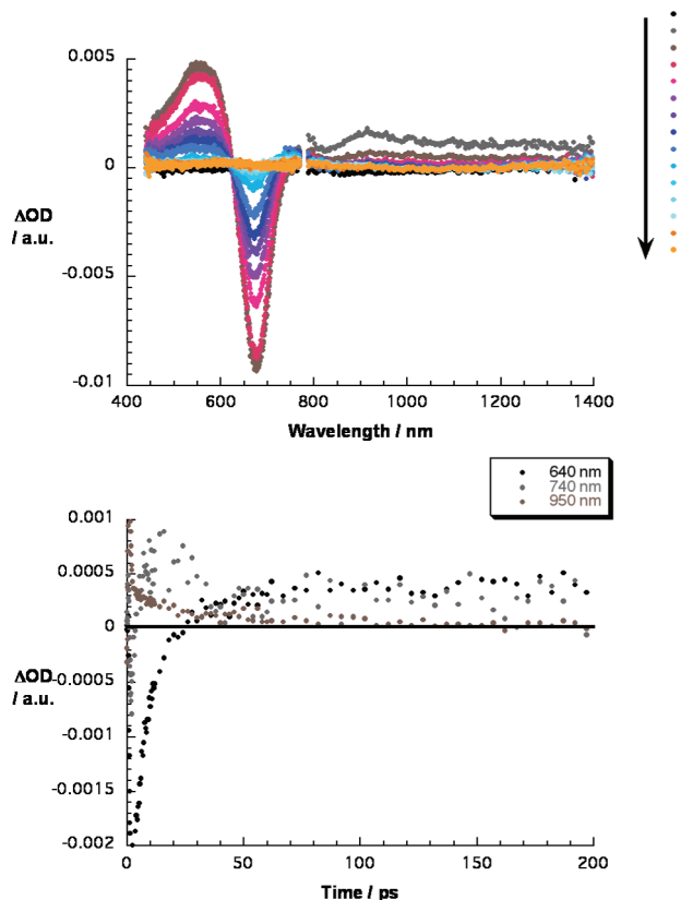
Figure 5. Time-resolved photophysical data for 2b . (Upper panel) Differential absorption spectra (visible and near-infrared) obtained upon femtosecond flash photolysis (388 nm - 200 nJ) of 2b ( 10^{-6} M) in THF with several time delays between 0 and 50 ps at room temperature; see legend for details about the time progression. (Lower panel) Time-absorption profiles of the spectra shown above at 640, 740, and 950 nm.
