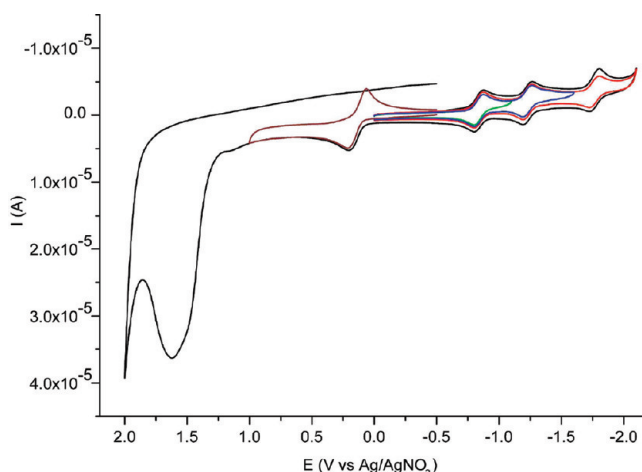
Figure 1. Cyclic voltammograms of 13 (~0.3 mM) in o -dichlorobenzene/acetonitrile (4:1) utilizing 0.1 M \text{Bu}_4\text{NClO}_4 as the supporting electrolyte and a glassy carbon as the working electrode at a scan rate of 100 \text{mV s}^{-1} .
