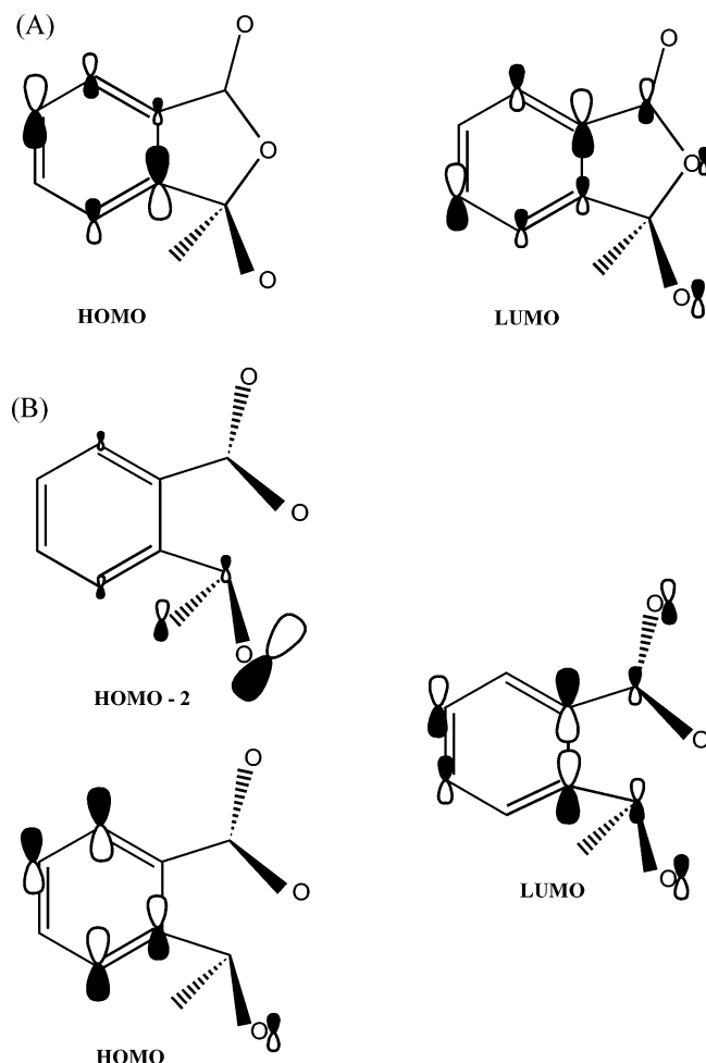
Figure 5. (A) Shape of orbitals involved in S_0 \rightarrow S_1 electronic excitation for the closed form ( R' ). (B) Shape of orbitals involved in S_0 \rightarrow S_1 electronic excitation for the open form ( O_3'' ).
