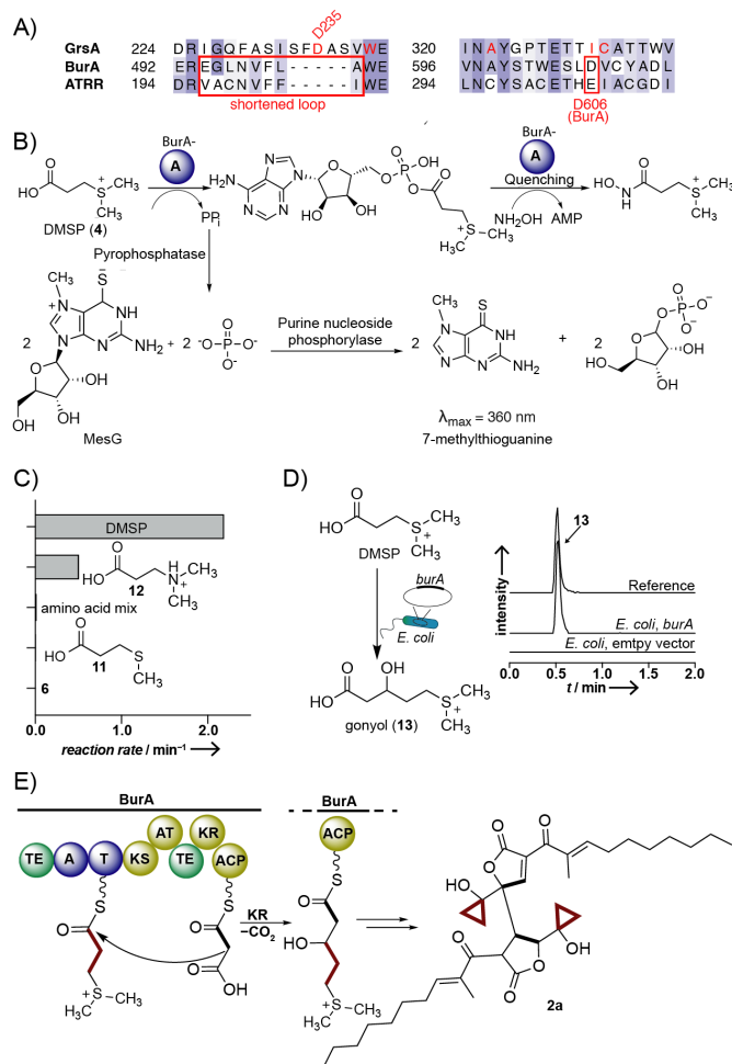
Figure 4. A) Sequence alignment of BurA-A with the canonical A domain GrsA and the glycine betaine accepting A domain ATRR. B) Concept of the MesG/hydroxylamine A domain assay C) Specificity profile of BurA-A; amino acid mix: all 20 proteinogenic amino acids (Supplementary Figure S6). D) Heterologous production of gonyol in E. coli ; UHPLC-MS monitoring: EIC ( m/z 179.0736) in positive ion mode; top, synthetic reference, middle, culture extracts of E. coli Rosetta2 expressing burA on plasmid pHIS8; bottom, E. coli Rosetta2 with empty pHIS8. E) Loading of DMSP onto BurA leads to production of gonyol and malleicypols.
