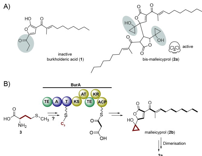
Figure 1. A) Structures of burkholderic acid (1) and bis-malleicyprol (2a) featuring a cyclopropanol warhead. B) Isotope-labeling studies [10] suggest acetate and methionine (3) as precursors to malleicyprol (2b), the monomer [11] of 2a.
