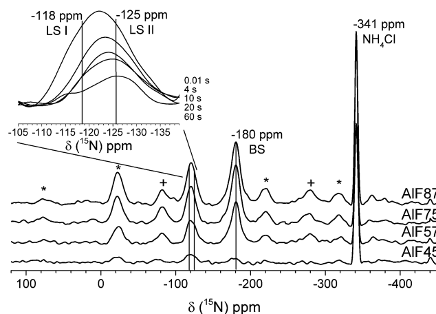
Fig. 5 ^{15}\text{N} NMR spectra of the four aluminum hydroxide fluoride samples loaded with ^{15}\text{N} -pyridine. The insert shows the Torchia spectra of AlF87 at different waiting times. The rotational side band of the Brønsted (+) and Lewis sites (*) are denoted.
