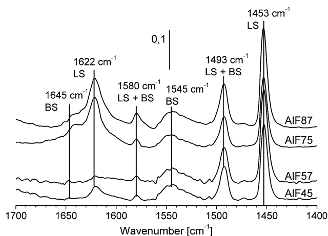
Fig. 4 FTIR spectra of the aluminum hydroxide fluoride samples after stepwise pyridine adsorption and desorption of excess pyridine. The spectra of AlF45 and AlF57 are magnified by a factor of five.
