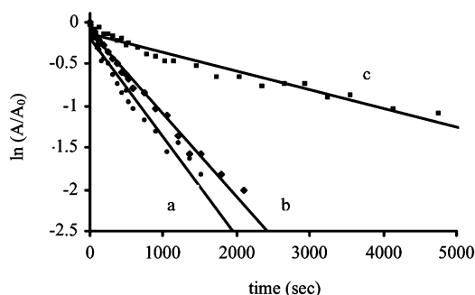
Fig. 3 Plot of \ln(A/A_0) versus time absorbance decay of photochromic peak for the host–guest complexes: (a) \gamma -CD-1, (b) \gamma -CD-2, (c) \gamma -CD-3.
