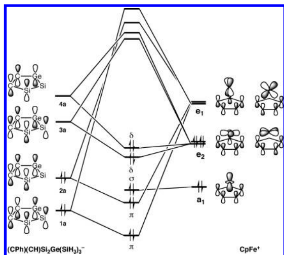
Figure 2. MO correlation diagram for the interaction between the model heavy Cp ligand [(\text{CPh})(\text{CH})\text{Si}_2\text{Ge}(\text{SiH}_3)_3]^- and the \text{CpFe}^+ fragment.
