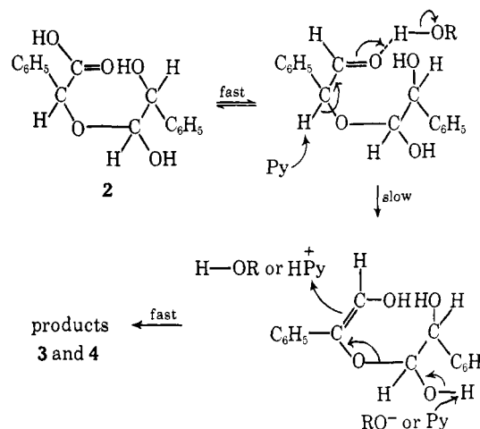
Scheme I. General Base-General Acid Catalyzed Isomerization of Mandelaldehyde
