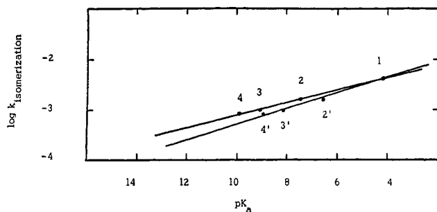
Figure 5. Brønsted correlation: 1, benzoic acid; 2, phenol ( pK_a correction 2.5); 2', phenol ( pK_a correction 3.4); 3, 2-pyridone ( pK_a correction 2.5); 3', 2-pyridone ( pK_a correction 3.4); 4, 4-trifluoroethanol ( pK_a correction 2.5); 4', trifluoroethanol ( pK_a correction 3.4).
