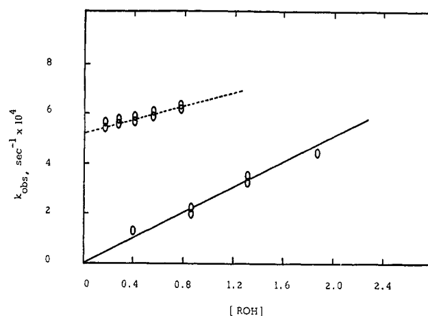
Figure 2. The dependence of the pseudo-first-order rate constant for the isomerization of 1-deuteriomandelaldehyde in pyridine at 90° on the equivalent concentration of the substrate plus product (—) and on the molar concentration of water (---).
