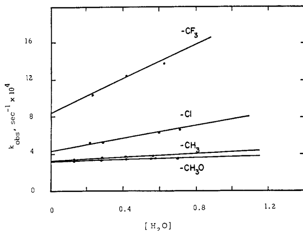
Figure 3. The dependence of the pseudo-first-order rate constants for the isomerization of substituted mandelaldehydes on the molar concentration of water (initial concentration of mandelaldehyde = 1.0 N).
