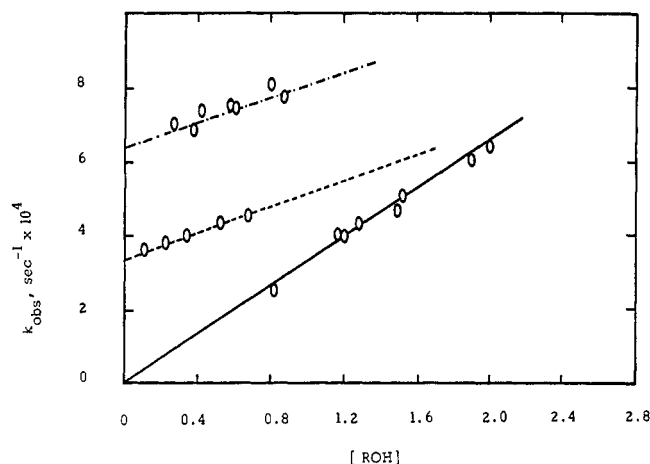
Figure 1. The dependence of the pseudo-first-order rate constant for the isomerization of mandelaldehyde in pyridine at 90° on the total substrate plus product concentration (—), on water concentration with mandelaldehyde concentration = 0.1 N (---), and on water concentration with mandelaldehyde concentration = 0.2 N (- · - · -).
