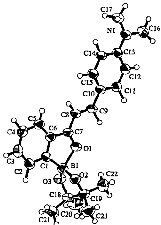
Figure 5 An ORTEP Drawing of 7
