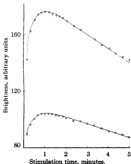
Fig. 5.—Time lag of stimulated emission of 100SrSe (0.020Sm, 0.020Eu) (6SrSO 4 , 6CaF 2 ).
