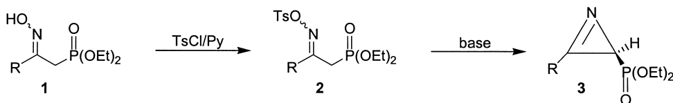
Scheme 2. 2 H -Azirines formation through modified Neber reaction of tosyl ketoximes 2
