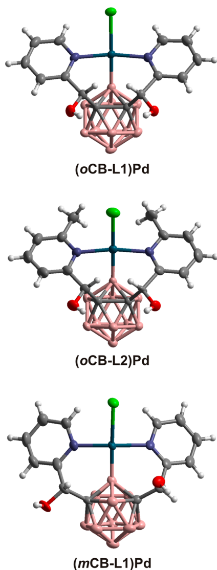
Figure 2. Molecular structures of (oCB-L1)Pd, (oCB-L2)Pd, and (mCB-L1)Pd; thermal ellipsoids set at 90%, 70%, and 80% probability, respectively, and H atoms are represented as fixed-size spheres of 0.18 Å (B–H and pyridine hydrogen atoms are omitted for clarity). Color code: B pink; C gray; H white; O red; N blue; Cl green; Pd prussian blue. Only one stereoisomer is represented in those structures with disorder of OH groups.
