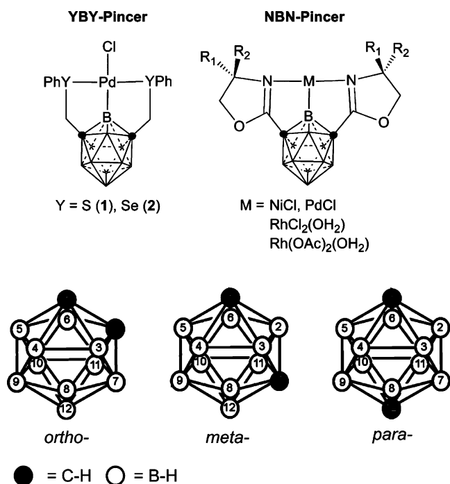
Figure 1. Reported closo -carboranyl-based pincers (top) and graphical representation of the carborane isomers ( closo -C 2 B 10 H 12 ) with vertex numbering.
