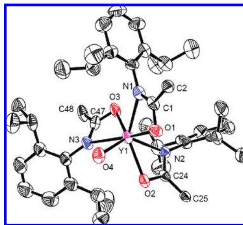
Figure 1. Oak Ridge Thermal Ellipsoid Plot (ORTEP) diagram of the solid-state molecular structure of [(\text{THF})\text{Y}(\text{Nap}[\text{O},\text{N}](i\text{-Pr})_2\text{Ph})_2]_2 ( 4 ) with the probability ellipsoids drawn at the 50% level. Naphthyl groups (except for ipso -carbon) and the carbons of the THF groups omitted for clarity. 65
