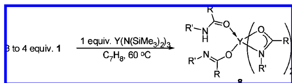
Scheme 2. Formation of Complex 8
