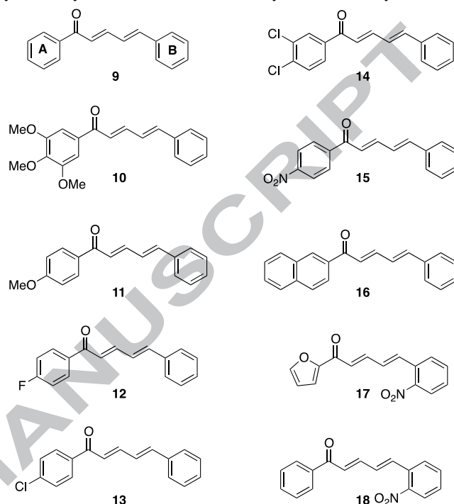
Figure 2. The library of cinnamylidenacetophenones synthesized for biological evaluation.
