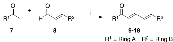
Scheme 2. Construction of target molecules 9-18 . (i) NaOH, H 2 O/EtOH (50% v/v), rt, 24h, 65-83%.
