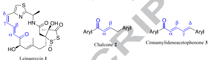
Figure 1. The development of cinnamylideneacetophenones from common features of leinamycin and chalcone skeleton.
