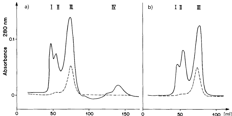
Fig. 1. Gel filtration (—) of the partially aggregated dimers on Sephadex G50 in 0.2 M \text{NH}_4\text{OAc} and rechromatography (---) of Peak III (in each case) under the same conditions. a) Dimer 7 ; b) dimer 10 .
