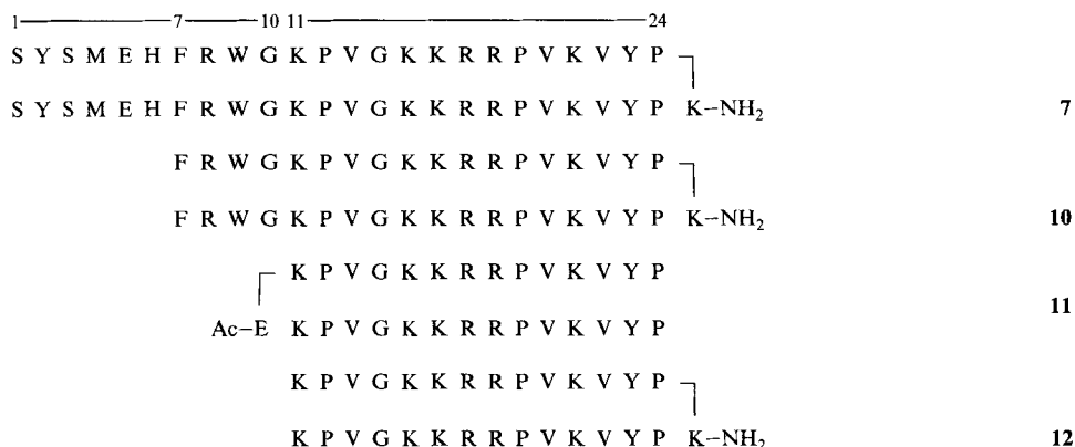
Fig. 2. Structure formula (see [1]) of the dimeric agonist 7 (this work) and of the dimeric antagonists 10 (this work) and 11 and 12 [4] [6]
